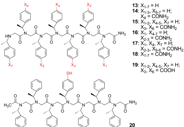
Figure 2. Synthesis of functionalized peptoid heptamers.
